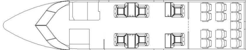
DHC-8-200 with 6 VIP/13 Economy
