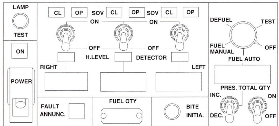
Ⓐ REFUEL/DEFUEL CONTROL PANEL
